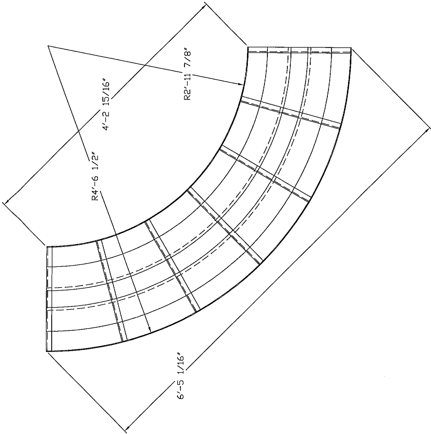
C121241-X91 RADIUS ROLL DETAIL
